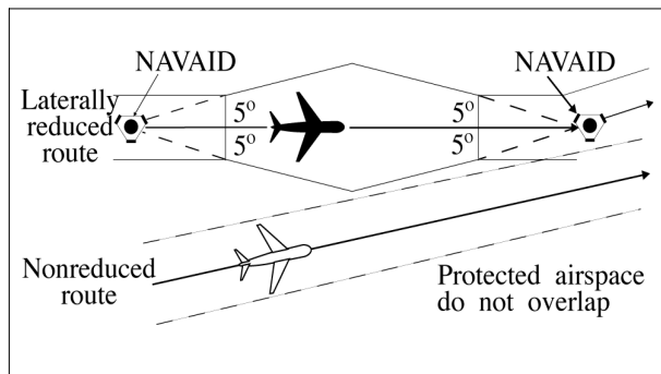
FIG 8-4-2 Separation Methods
