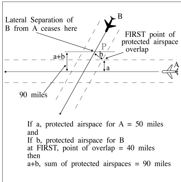
FIG 8-4-6 Separation Methods
