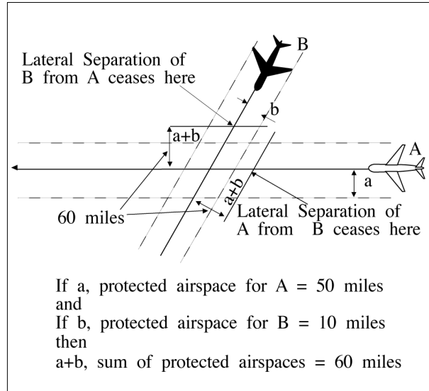
FIG 8-4-5 Separation Methods
