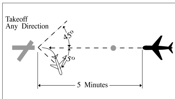
FIG 6-3-2 Separation Minima
