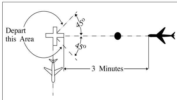
FIG 6-3-1 Separation Minima
