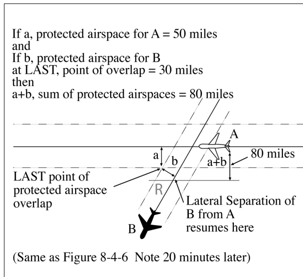
FIG 8-4-7 Separation Methods
