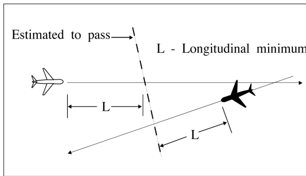
FIG 8-3-3 Reciprocal Courses
