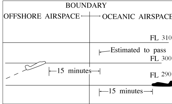
FIG 8-5-2 Transitioning From Offshore to Oceanic Airspace Opposite Direction
